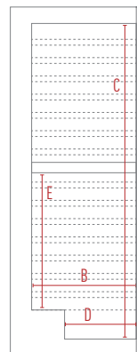
SLIM WINE SW 105 2TB LATO / SIDE
