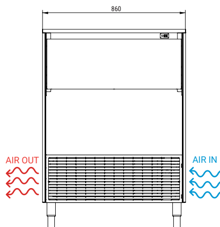
FRONTAL VIEW VISTA FRONTAL
