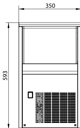
FRONTAL VIEW VISTA FRONTAL
