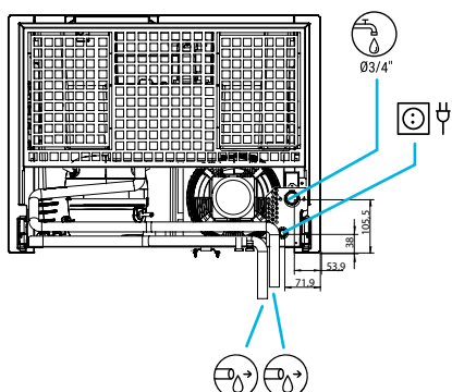
REAR VIEW VISTA TRASERA
