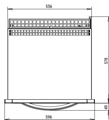
FLOOR VIEW VISTA PLANTA
