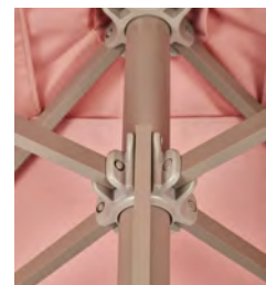
Ribs without screws for an easier replacement
