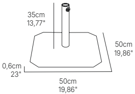
BSO500GR4503 ø45 grey
