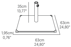
BSC625GR6010 ø60 grey
