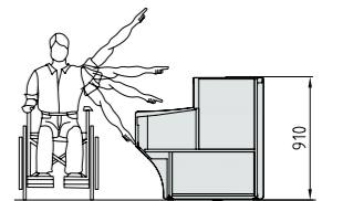
Servicio adaptado Service adapted Service adaptés
