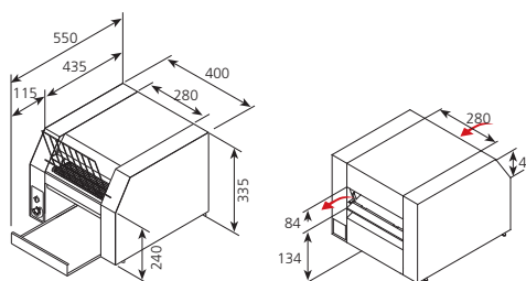
TPC-40
