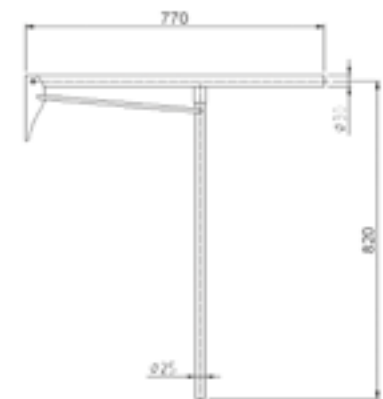
Asidero abatible 180° con pata Folding support rail with leg
